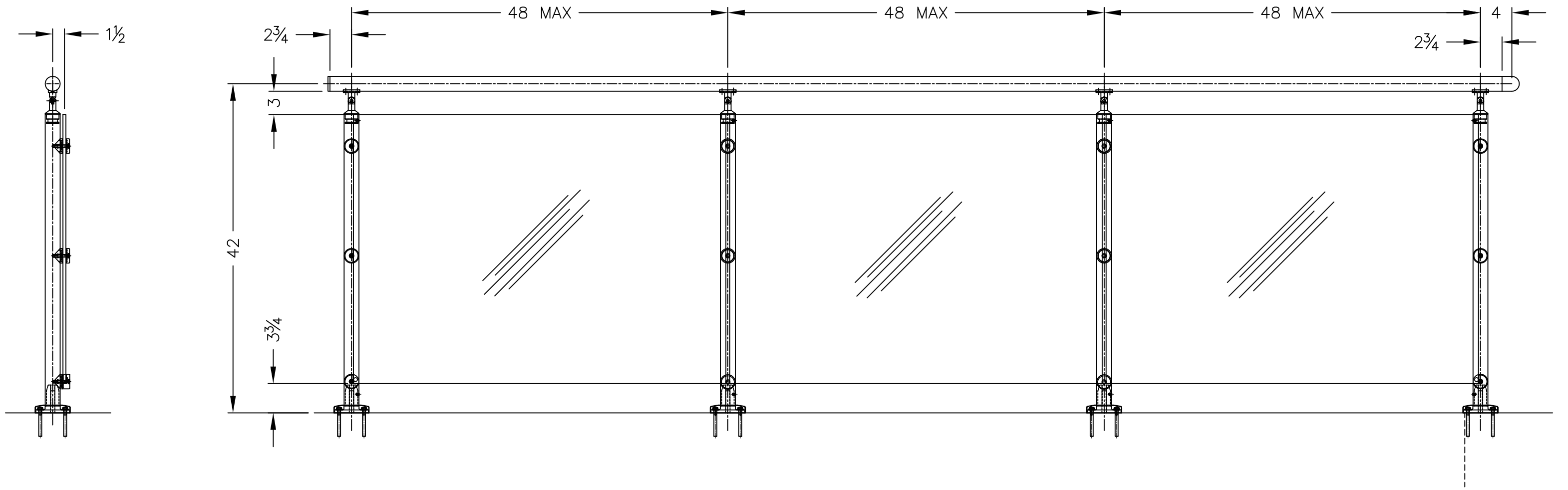
VUE RAIL - LEVEL (TOP MTG.) GUARD RAIL
